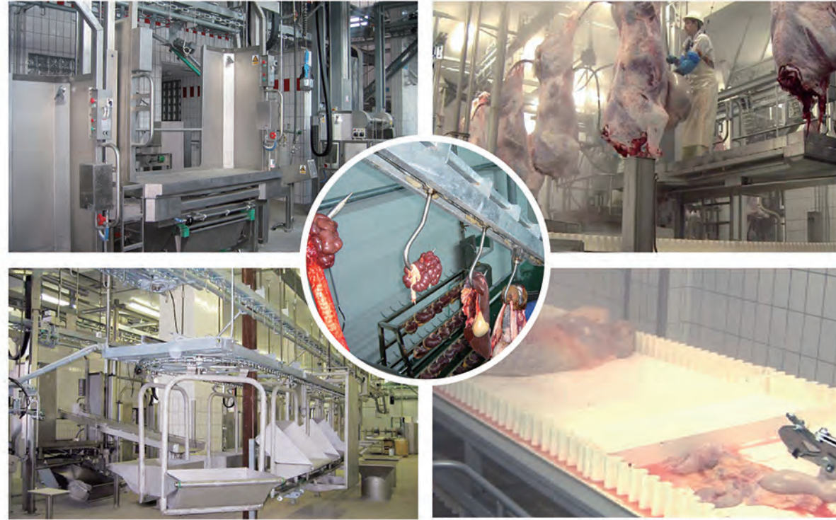
Pneumatic lift eviscerating 取内脏气动升降台
