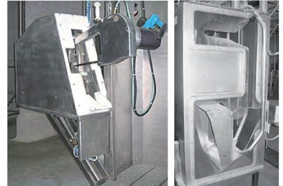
Washing & sterilizing device for pans, hooks and saws 盘, 钩, 锯清洗消毒装置
